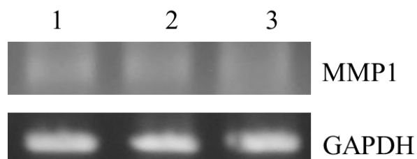
Fig 1: Effect of the Test Substance on MMP-1 transcripts in HDF Lane 1: Untreated Control, Lane 2: Test substance Green Tocyen beauty cream (RR222098) at 500 µg/mL, Lane 3: Test substance Tocyen beauty cream (RR222098) at 1000 µg/mL.
